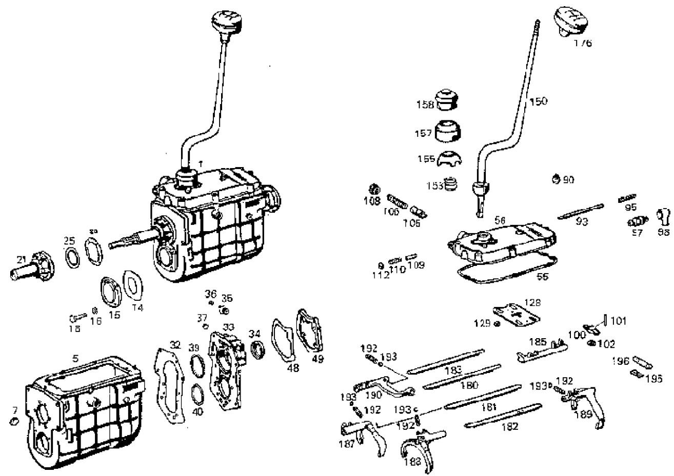
GBS 40 SYNCHROMESH TRANSMISSION
