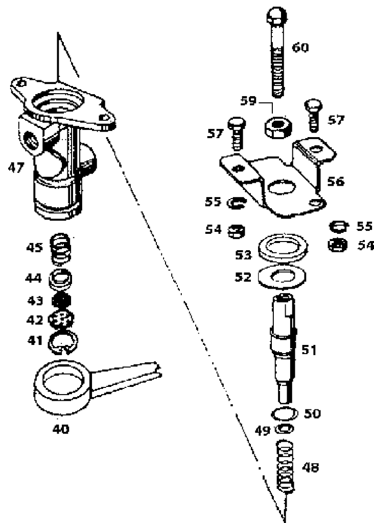
EXHAUST BRAKE VALVE
