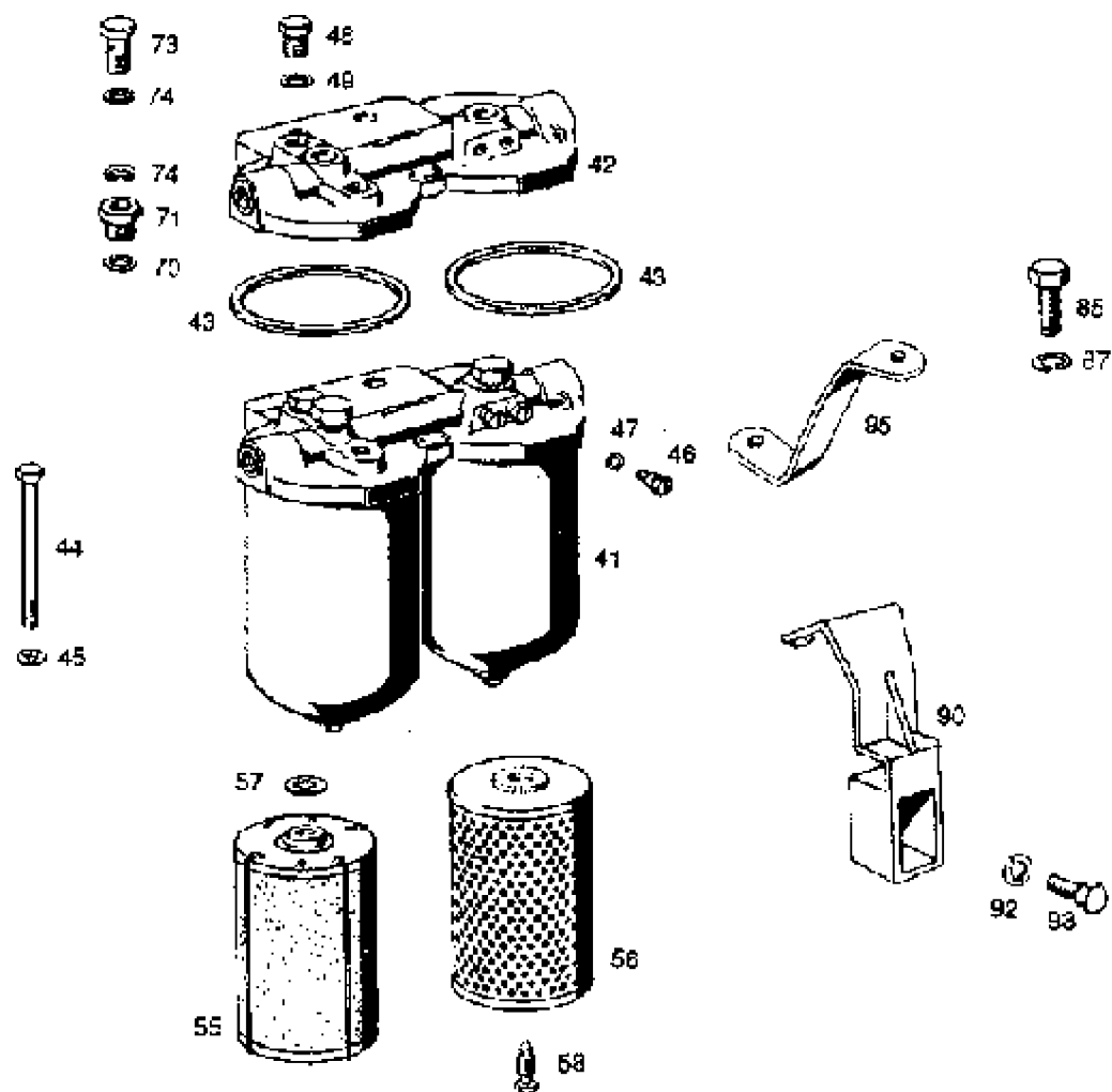
FUEL MULTISTAGE FILTER
