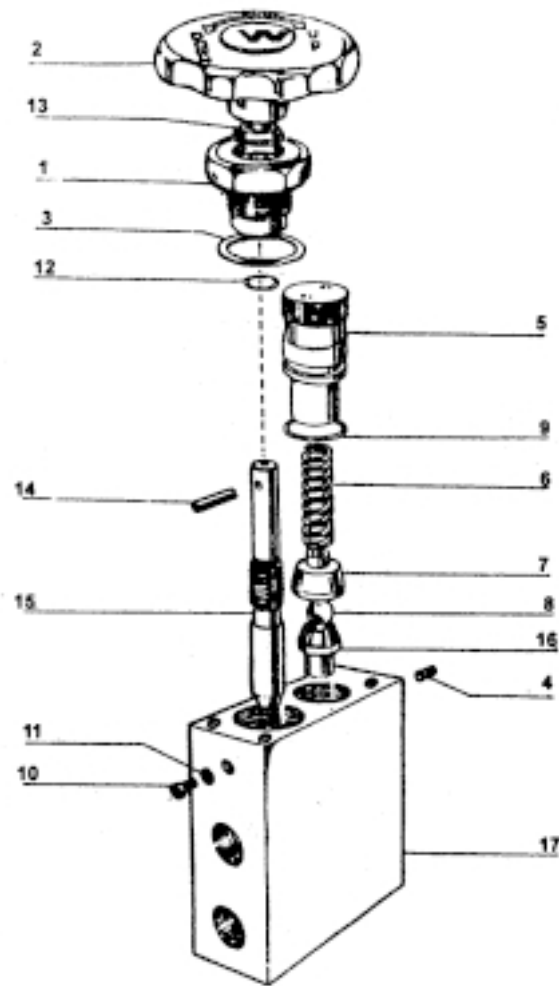
MANUAL VALVE ROTARY
