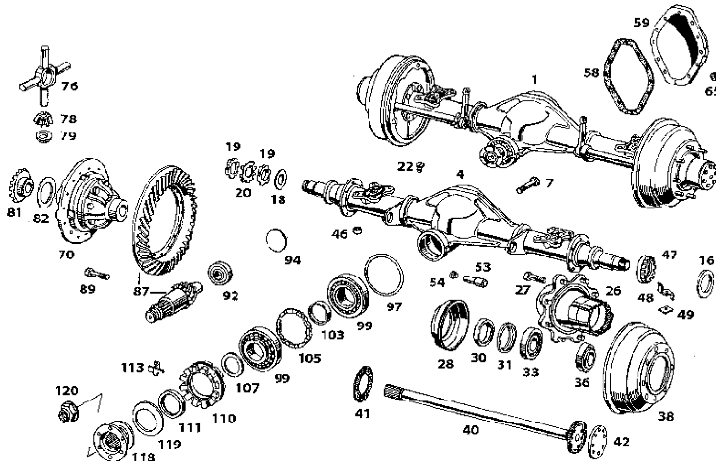
REAR AXLE (SALISBURY TYPE)
