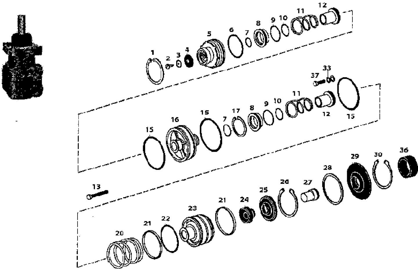
DUAL BRAKE VALVE
