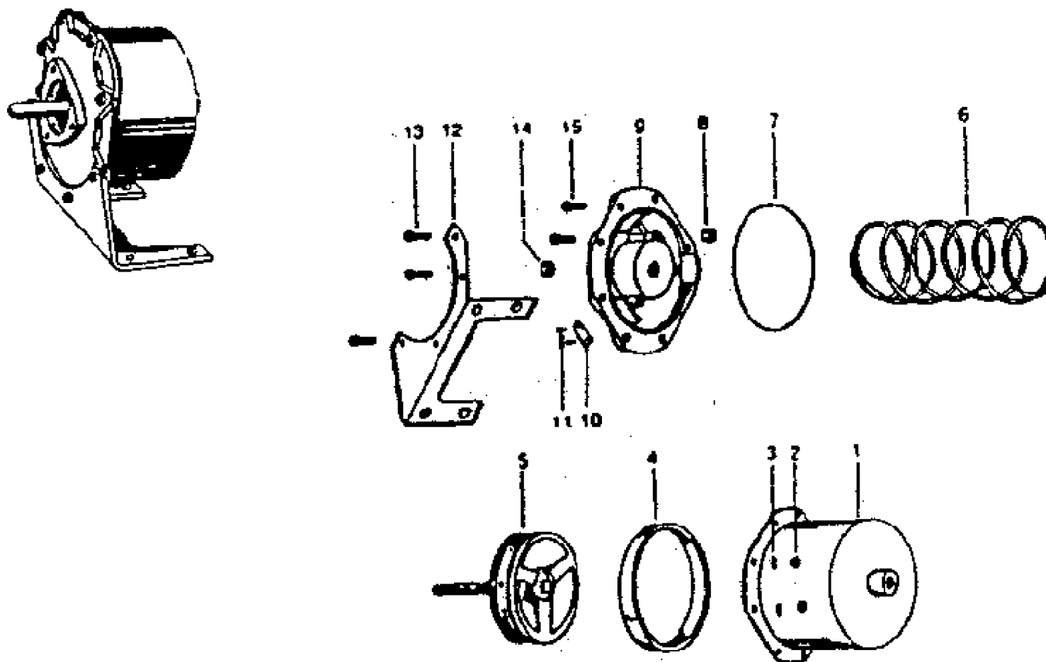
AIR CYLINDER
