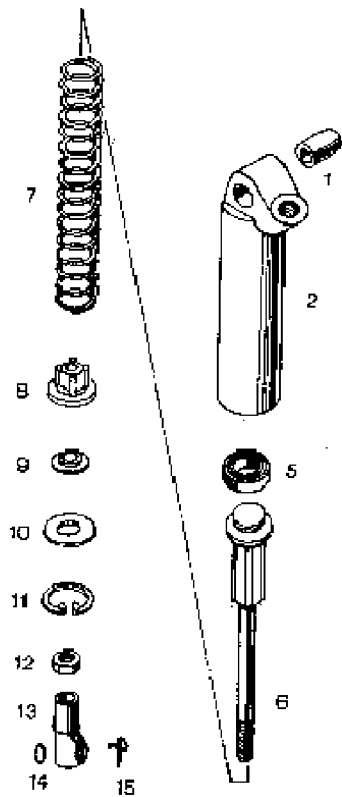
AIR CYLINDER
