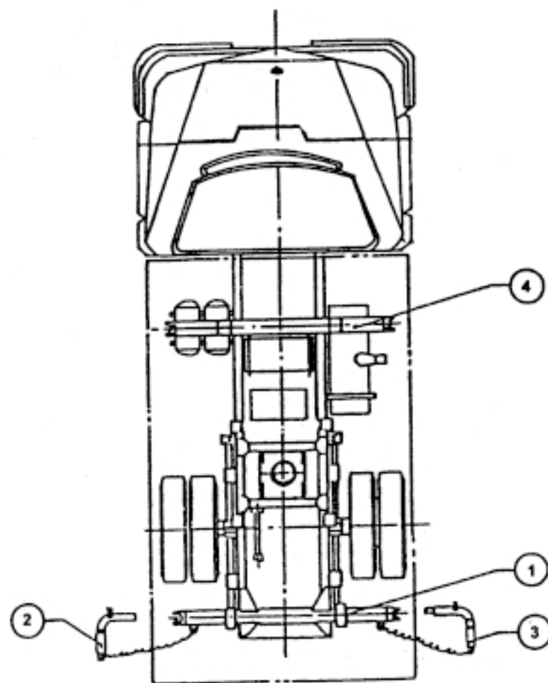
STABILITY SHAFT
