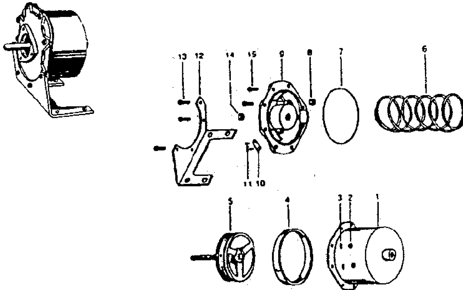
AIR CYLINDER
