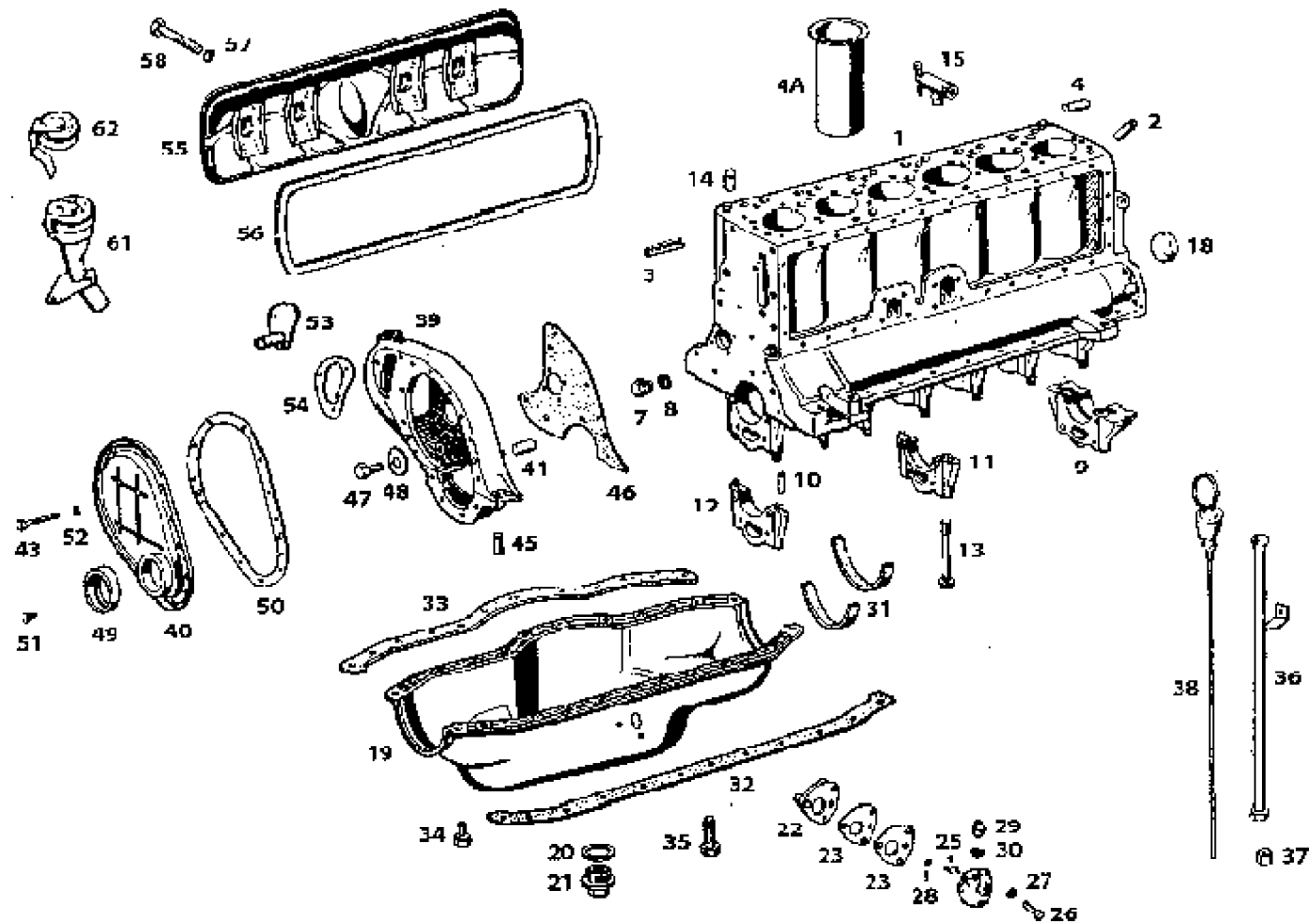
CYLINDER CRANK CASE
