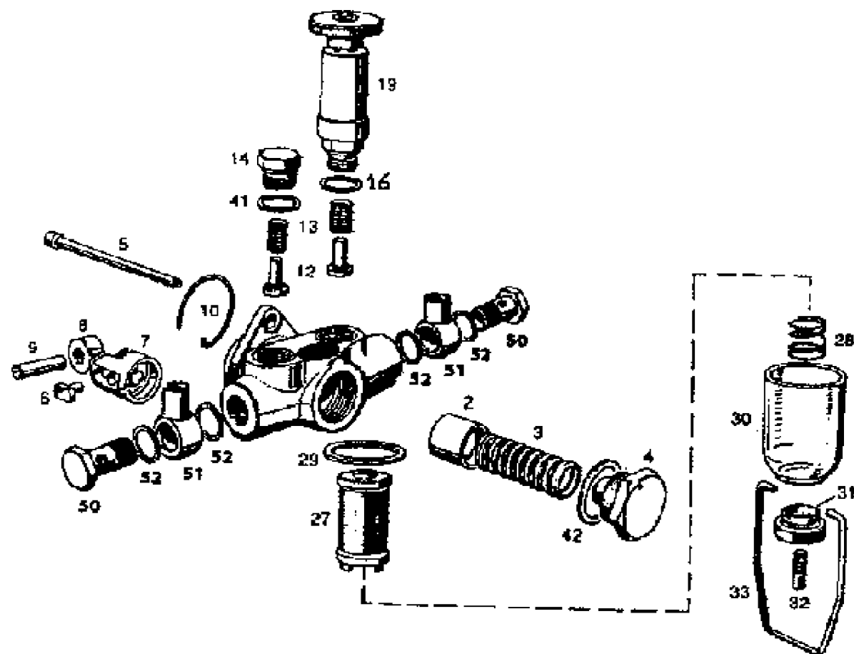
FUEL FEED PUMP
