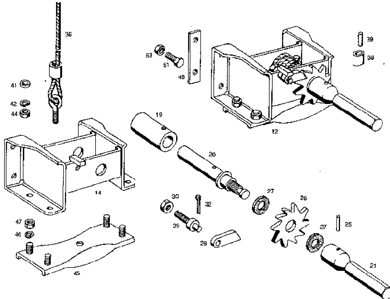
SPARE WHEEL CARRIER (WINCH TYPE)
