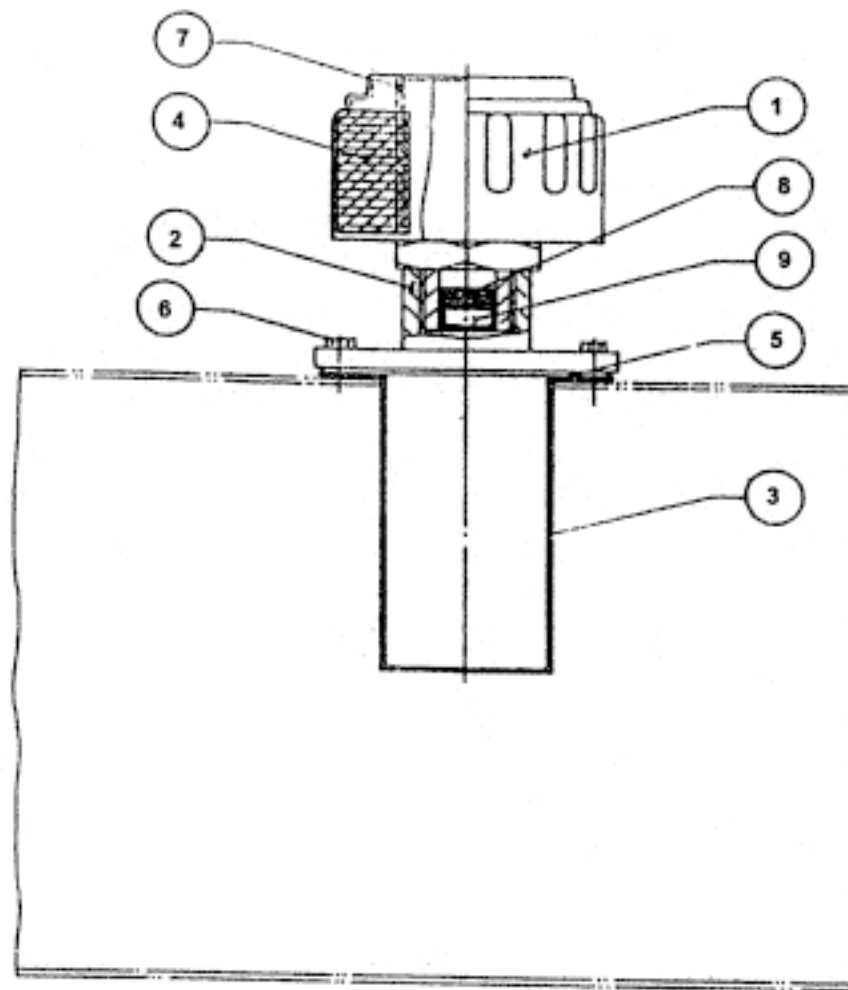
FILTER BREATHER
