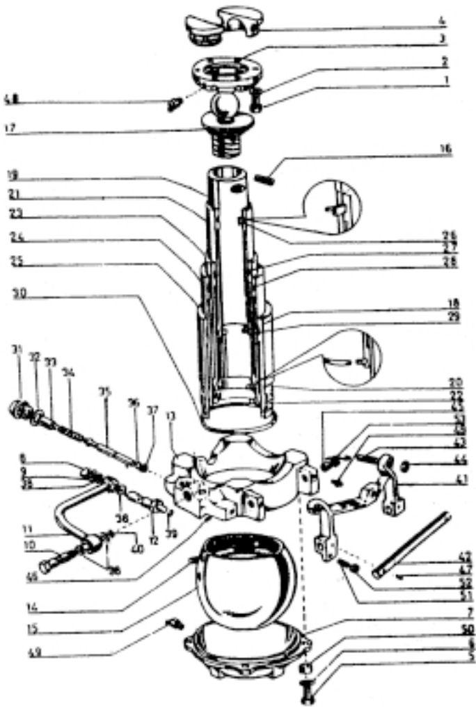
TELESCOPIC CYLINDER (4 STAGES)
