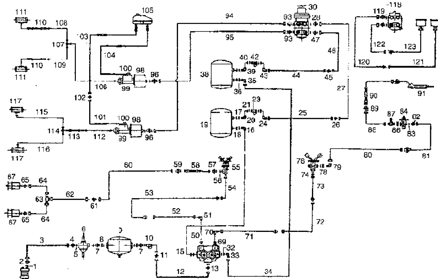
BRAKE LINES
