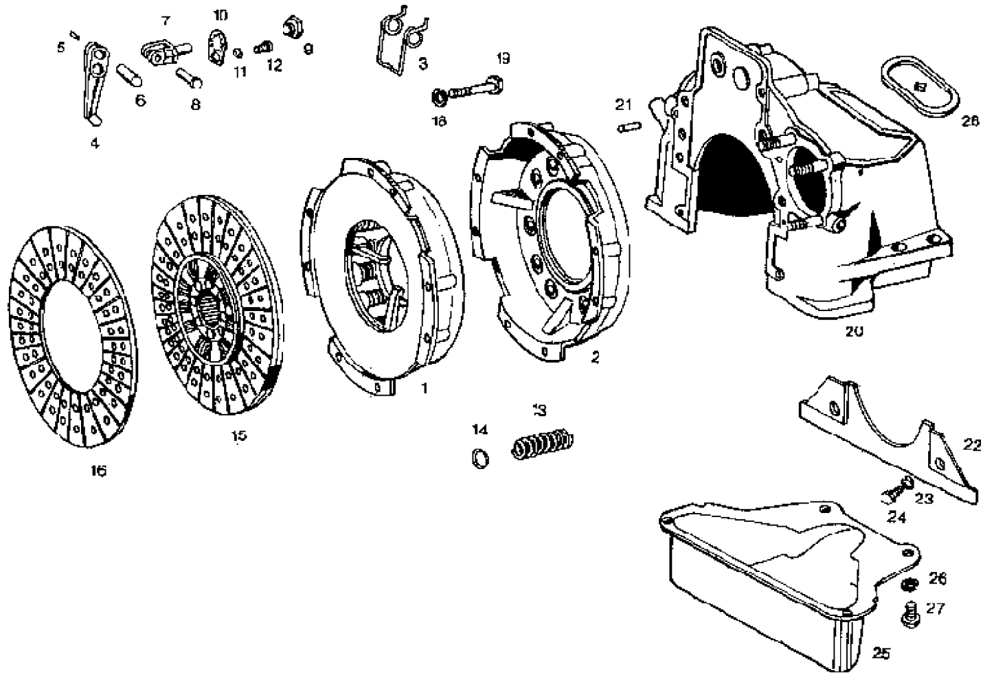
CLUTCH 310 MM DIA (COIL TYPE)
